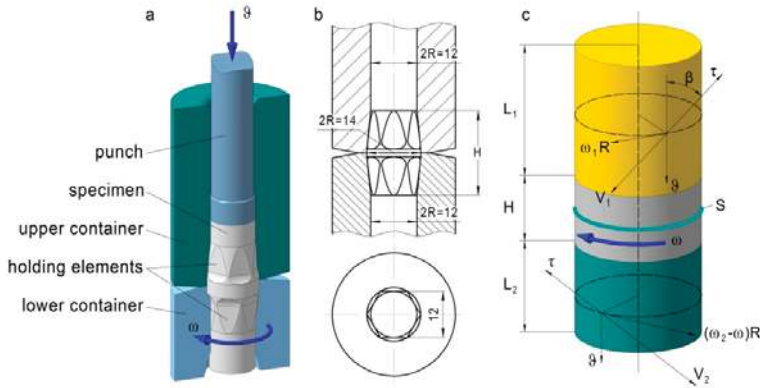
Figure 1. High pressure torsion extrusion: (a) schematics of the process, (b) design of containers and (c) definitions of the quantities for calculations. (unit: mm).
