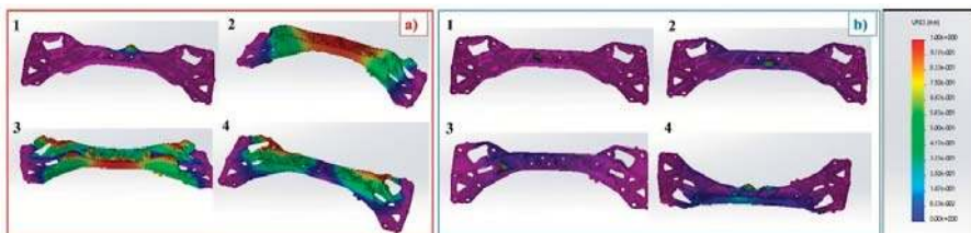
Figure 7. Displacement trend for the first four deformations for original geometry: (a) load case 1 (F); (b) load case 2 (M).
