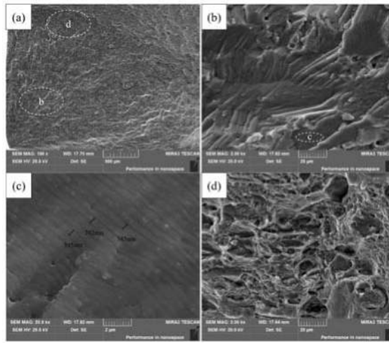
Figure 10. The fatigue fracture surfaces of A-Cu-Mg alloy under 210 MPa after 12 h of creep aging at 180 °C: (a) full view; (b) fracture nucleation; (c) stable fatigue crack growth; (d) final fracture.
