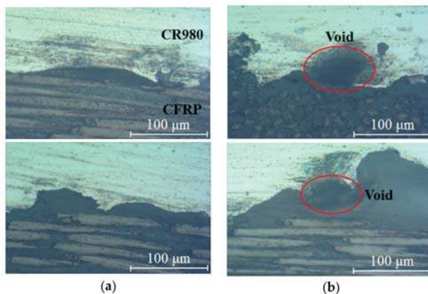
Figure 10. Microstructures (section view) CFRP/CR980 hybrid composites conducted by shear lap adhesion test: (a) surface roughness R_z = 45 \mu\text{m} ; (b) surface roughness R_z = 60 \mu\text{m} .
