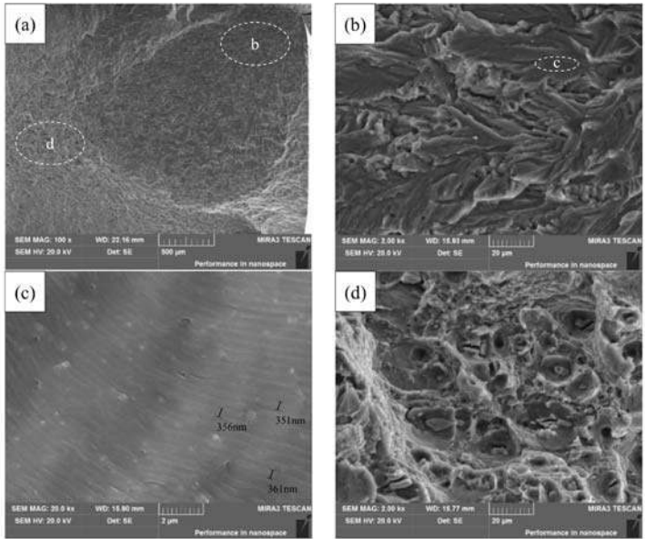
Figure 5. The fatigue fracture surfaces of Al-Cu-Mg alloy under 180 MPa after 12 h of creep aging at 160 °C: (a) full view; (b) fracture nucleation; (c) stable fatigue crack growth; (d) final fracture.
